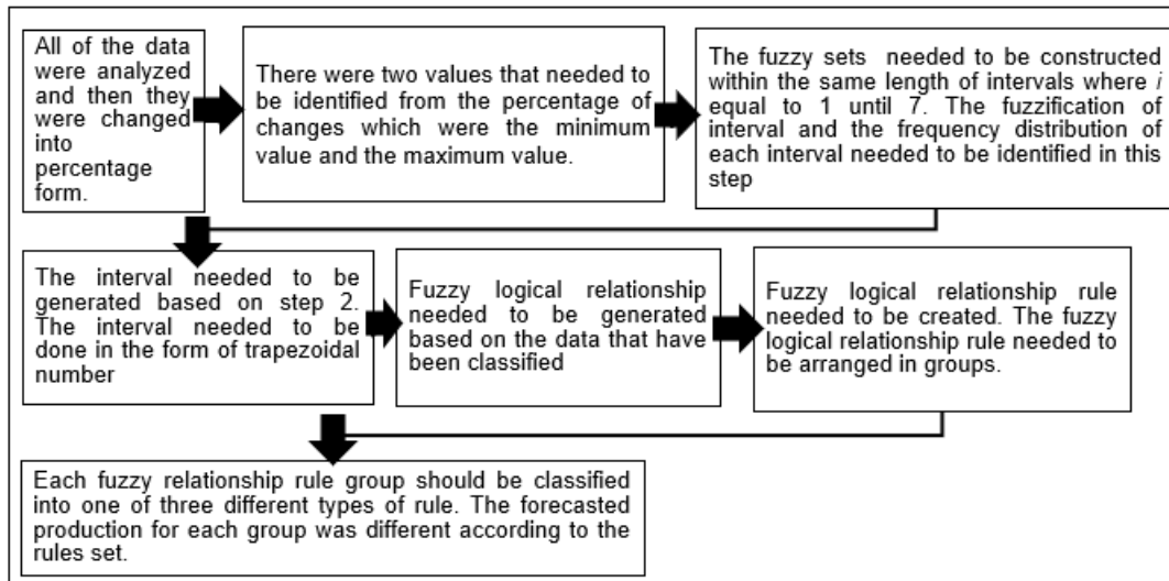
Figure 1: Step of Fuzzy Time Series
