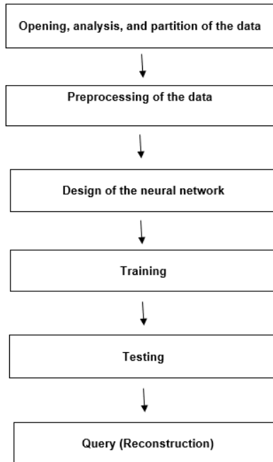
Figure 2: Steps of using Alyuda NeuroIntelligence Software
