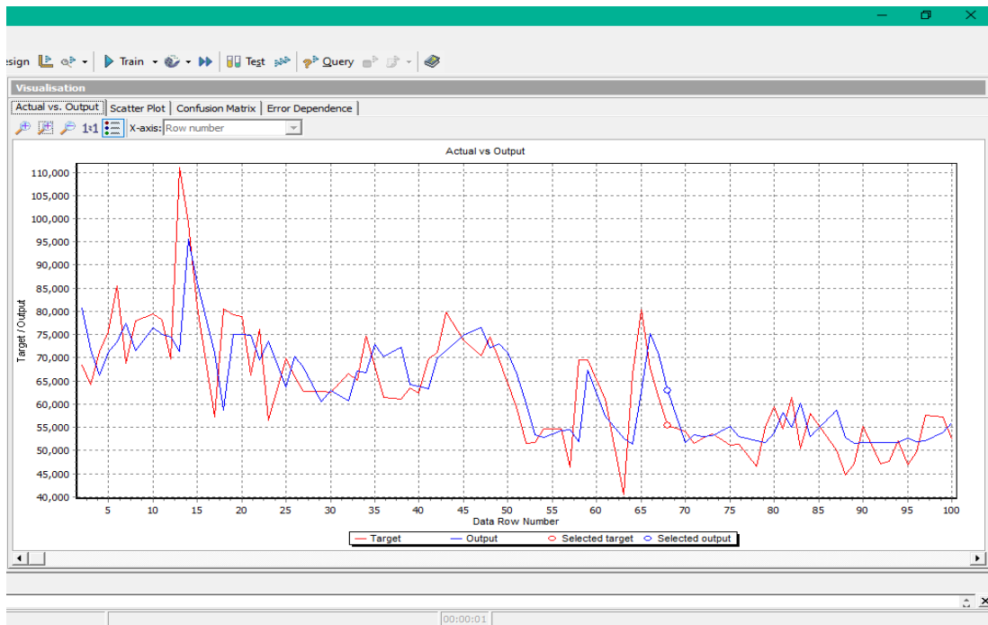
Figure 4: Graph of Actual versus Output based on Limited Memory Quasi-Newton
